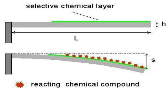
Fig. 7 Molecular adsorption induced bending a cantilever
