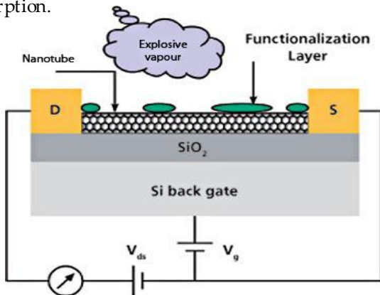
Fig. 6 Illustration of nano wires sensor platform
